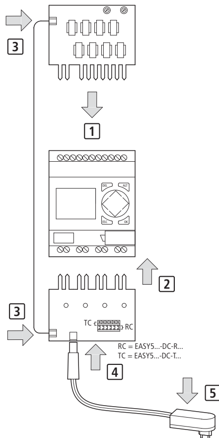
EASY412-DC-SIM: EASY512-DC-...
