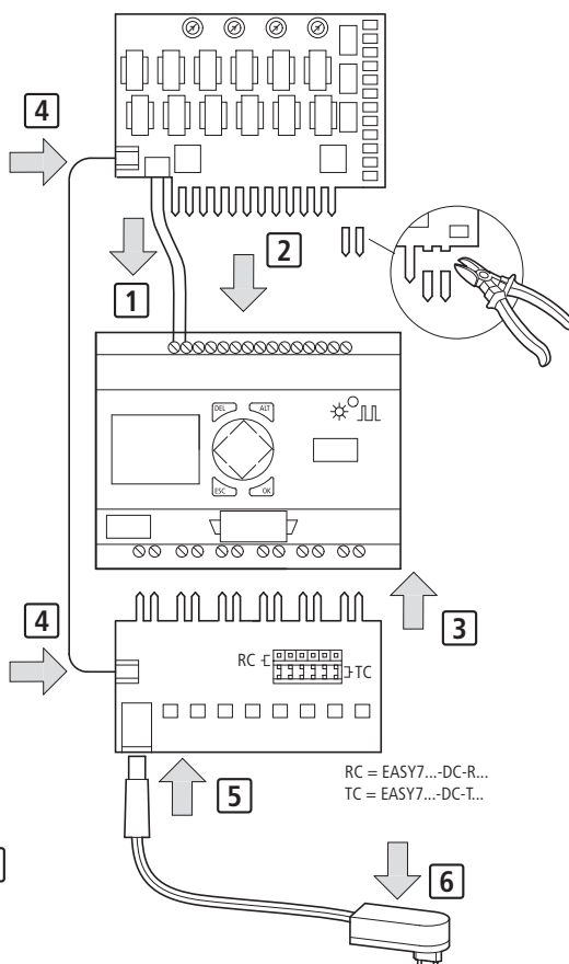
EASY800-DC-SIM: EASY7...-DC-...
