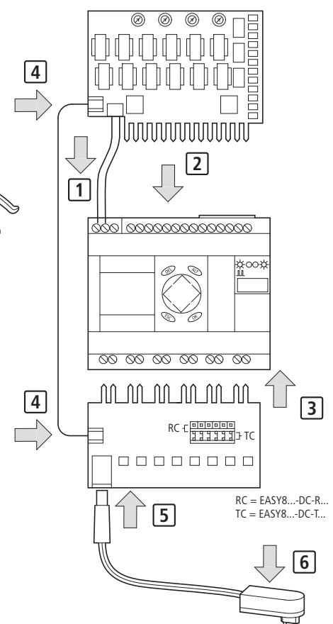
EASY800-DC-SIM: EASY8...-DC-...
