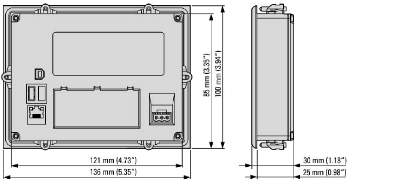
HMI-PLC SmartWire-DT
