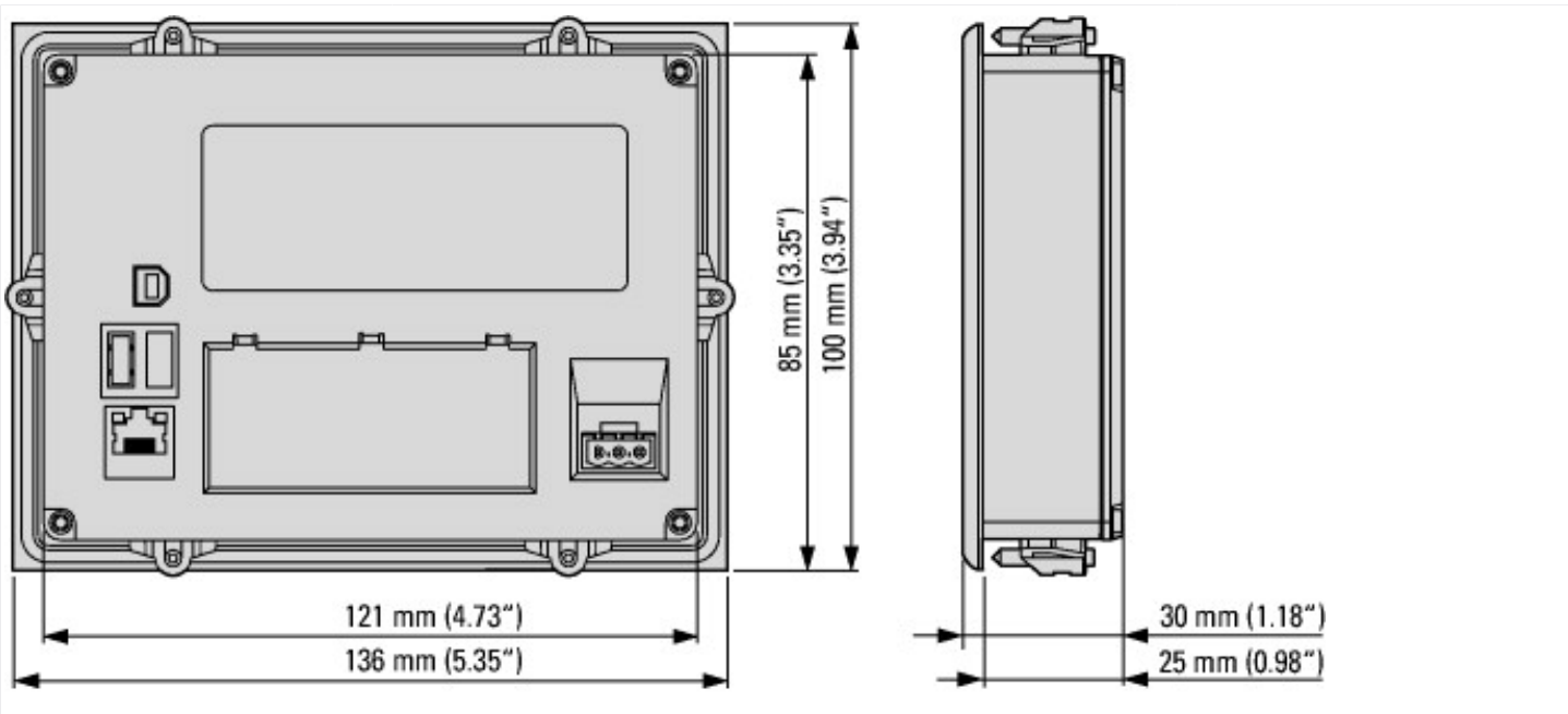
HMI-PLC SmartWire-DT
