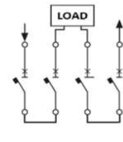
4 poles in series
