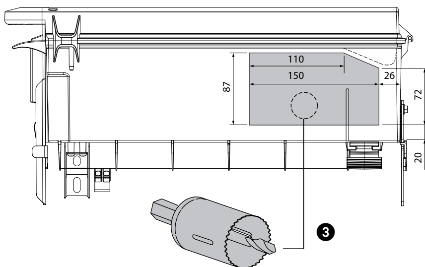
SIDE VIEW
