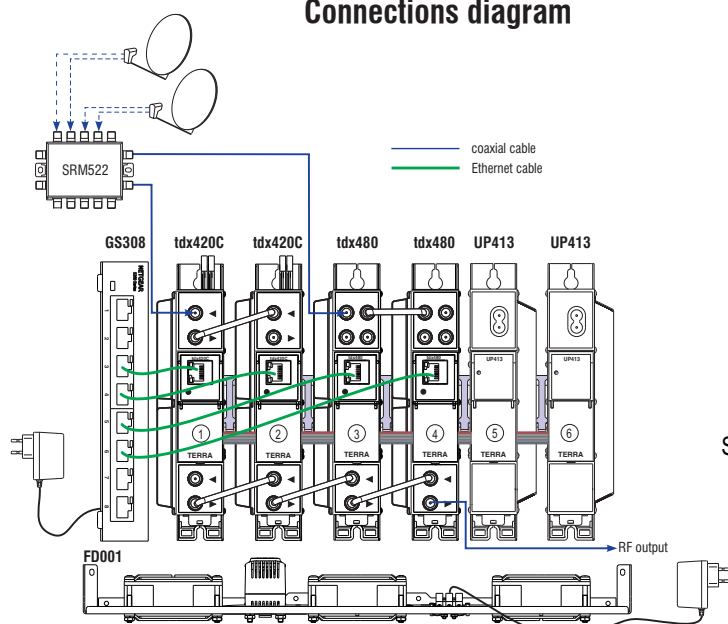
Connections diagram
